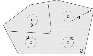
Fig. 2 Illustration of the median circling policy. The squares represent p^* , the m median of \mathcal{Q} . Each UAV loiters about its respective generator at a radius c_2\rho . The regions of dominance are demarcated according to the Voronoi partition generated by p^* . In this figure, a target has appeared in the subregion roughly in the upper-right quarter of the domain. The UAV responsible for this subregion has left its loitering station and is en route to service the target.
