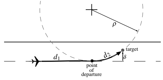
Fig. 5 Closeup of the strip loitering policy with construction of the point of departure and the distances \delta , d_1 , and d_2 for a given target, at the instant of appearance.
