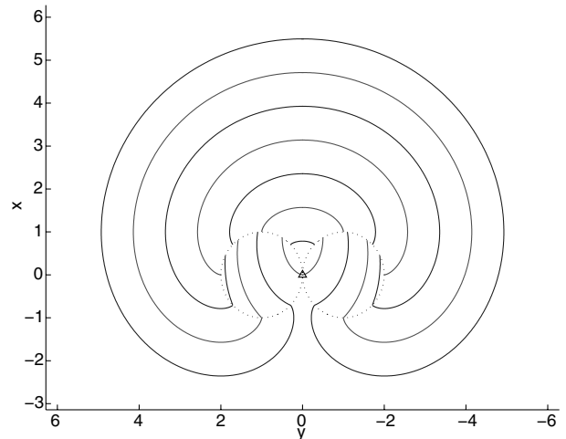
Fig. 13 The level sets of the function L_\rho(g_0, q) , for \rho = 1 , shown at increments of \pi/4 . The initial vehicle configuration is represented by the triangle and is at coordinates (0,0) heading up. Note that the positive direction of the x axis is up and of the y axis is left.
