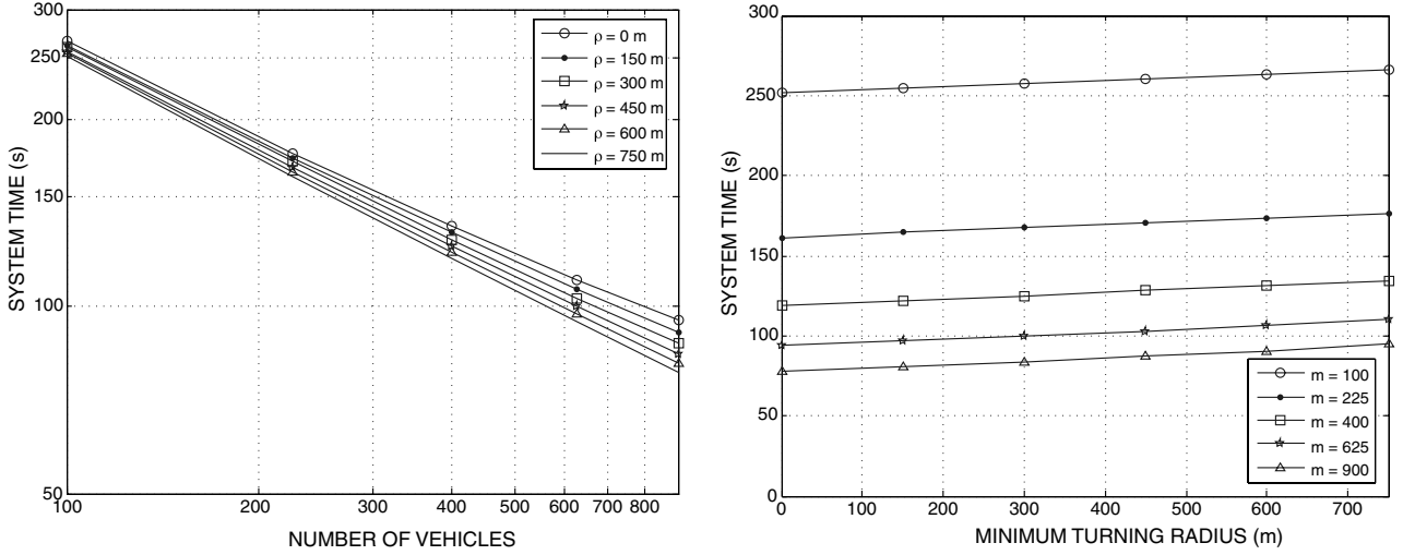
Fig. 3 Simulations of the MC policy were run with a square environment of area A = 9 \times 10^{10} \text{ m}^2 and vehicle speed v = 50 \text{ ms}^{-1} . The performance of the MC policy is plotted as a function of 1) the number of vehicles (left), and 2) the minimum turning radius of the vehicles (right). The nonholonomic vehicle densities for the scenarios of all data points shown lie within the range 0 \leq \rho \leq 0.0056 .
