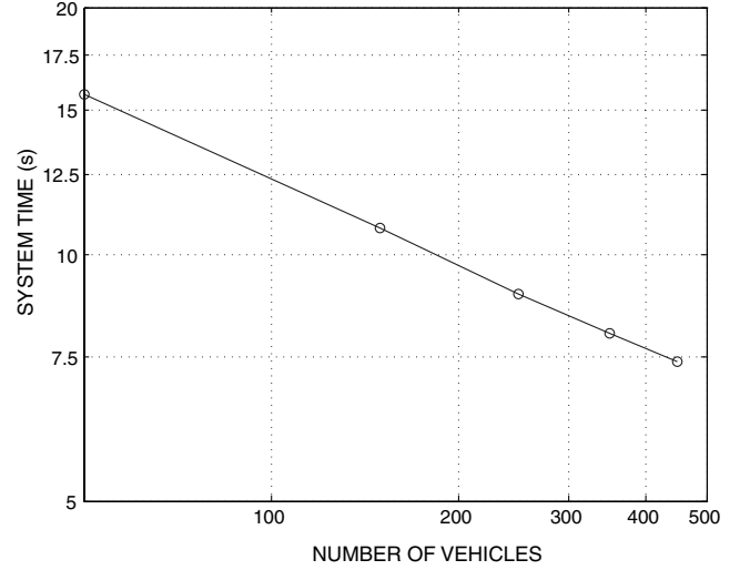
Fig. 6 Simulations of the SL policy were run with a square environment of area A = 9 \times 10^6 \text{ m}^2 , vehicle speed v = 50 \text{ ms}^{-1} , minimum-turning radius \rho = 600 \text{ m} , and m varying from 50 to 450. The nonholonomic vehicle densities for the scenarios of all data points shown lie within the range 2 \leq d_\rho \leq 18 .
