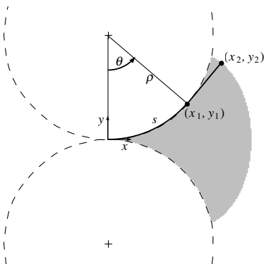
Fig. 1 The derivation of \text{area}(R_t(g_i)) for t \leq \pi\rho/(2v) .
