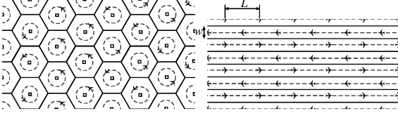
Fig. 11 The MC (left) and SL (right) policies with an infinite number of vehicles on an unbounded domain.
