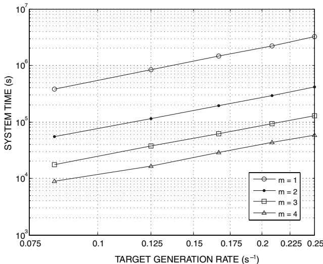
Fig. 9 Simulations of the mBT policy were run with a square environment of area A = 3.6 \times 10^7 \text{ m}^2 , vehicle speed v = 50 \text{ m s}^{-1} , minimum-turning radius \rho = 600 \text{ m} , number of vehicles m varying from 1 to 4, and target-generation rate \lambda varying from 1/12 to 1/4 \text{ s}^{-1} in increments of 1/24 \text{ s}^{-1} . Plots of the system time versus target-generation rate (left), and system time versus the number of vehicles (right) are given.
